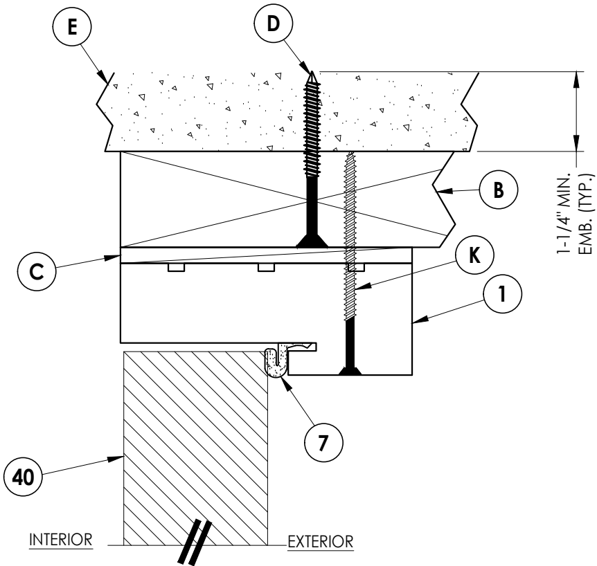
2 VERTICAL CROSS SECTION 5 2X Buck Construction
