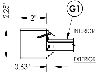
1/3 HORIZONTAL CROSS SECTION
