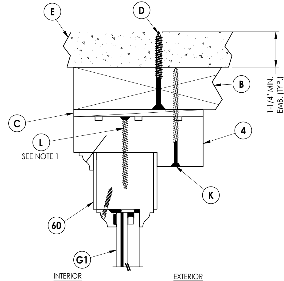
3 VERTICAL CROSS SECTION 5 2X Buck Construction
