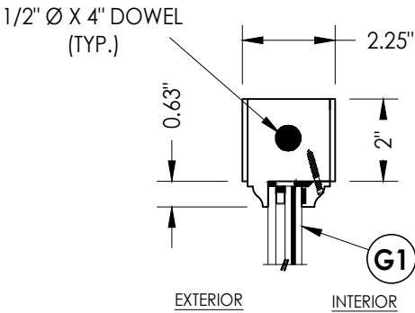
2/3 VERTICAL CROSS SECTION
