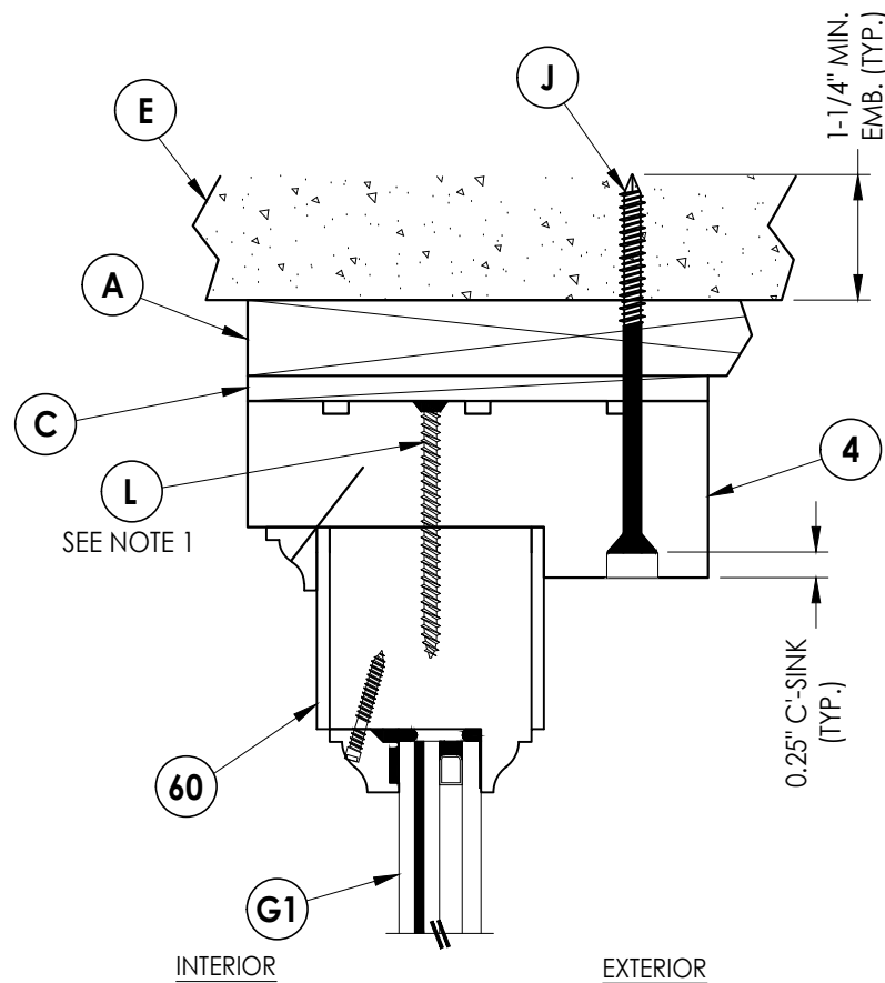
3 6 VERTICAL CROSS SECTION 1X Buck Construction
