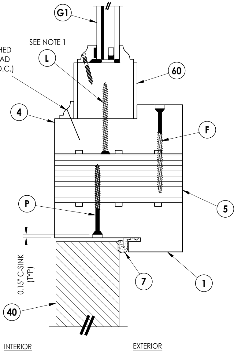
1 8 VERTICAL CROSS SECTION
