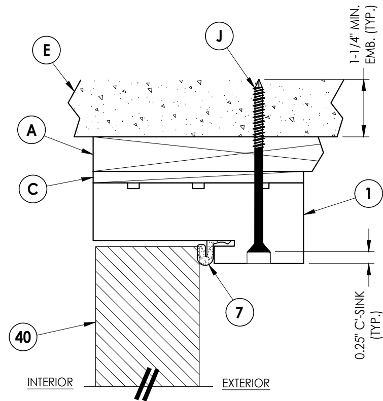
2 VERTICAL CROSS SECTION 6 1X Buck Construction
