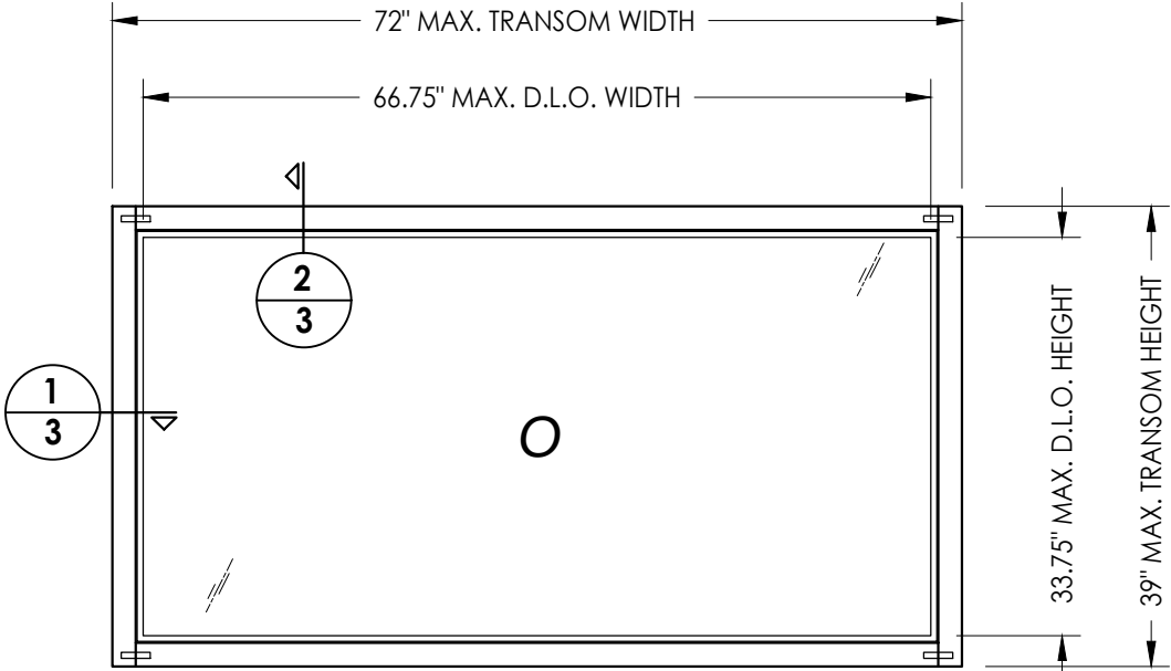
60 TRANSOM PANEL UPSTATE DOOR
