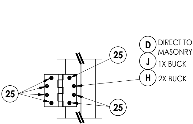
HINGE DETAIL
